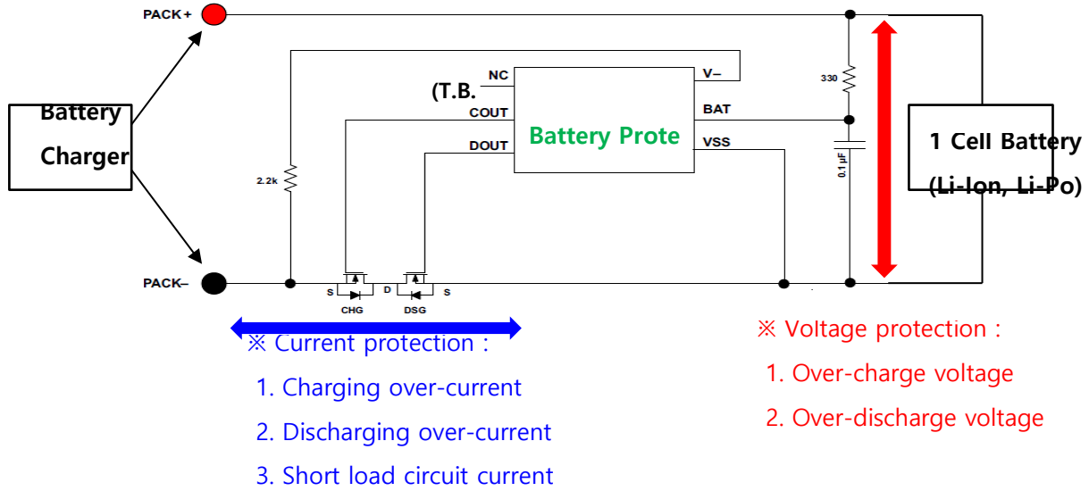
Figure 1 Block Diagram of BPIC)
